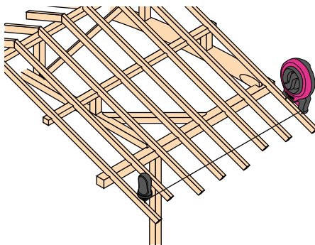
Finding Length of Rafter Edge
