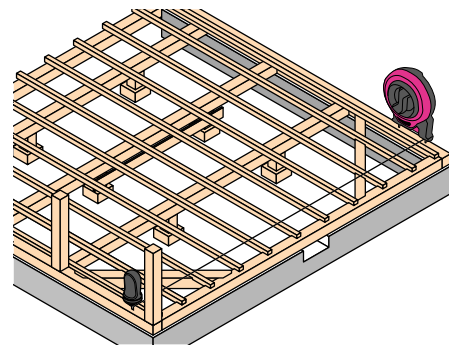
Adjusting Height of Joist
