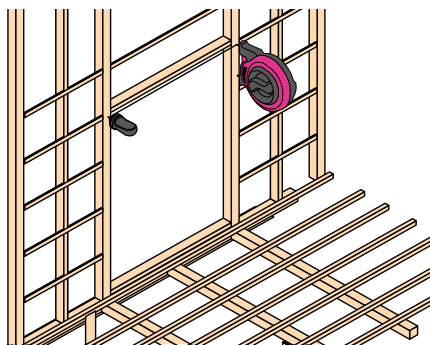
For leveling of lintel
